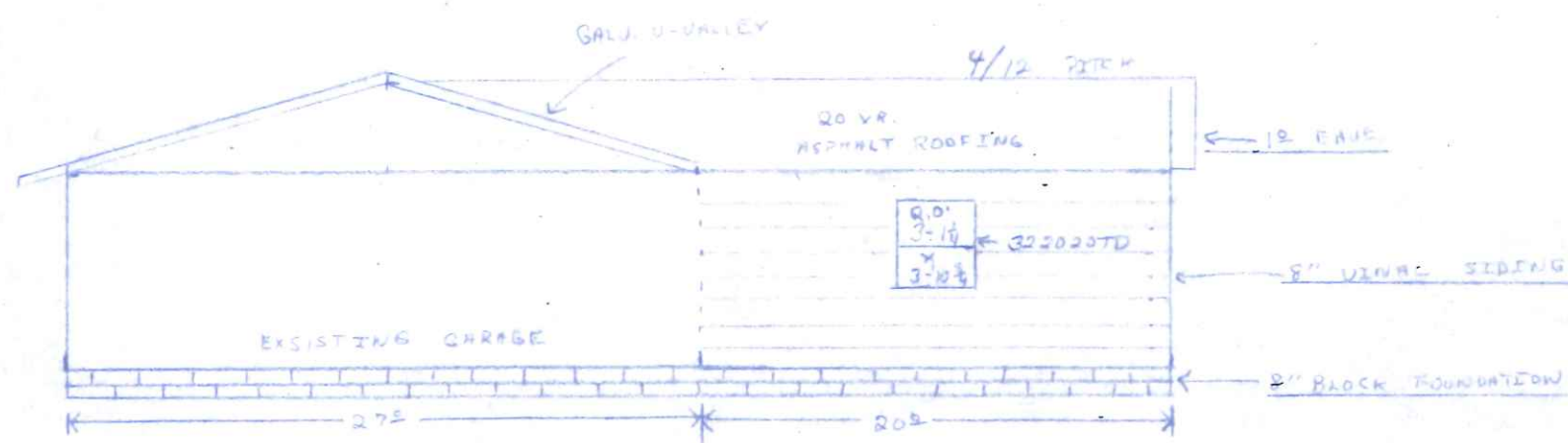
WEST ELEVATION
