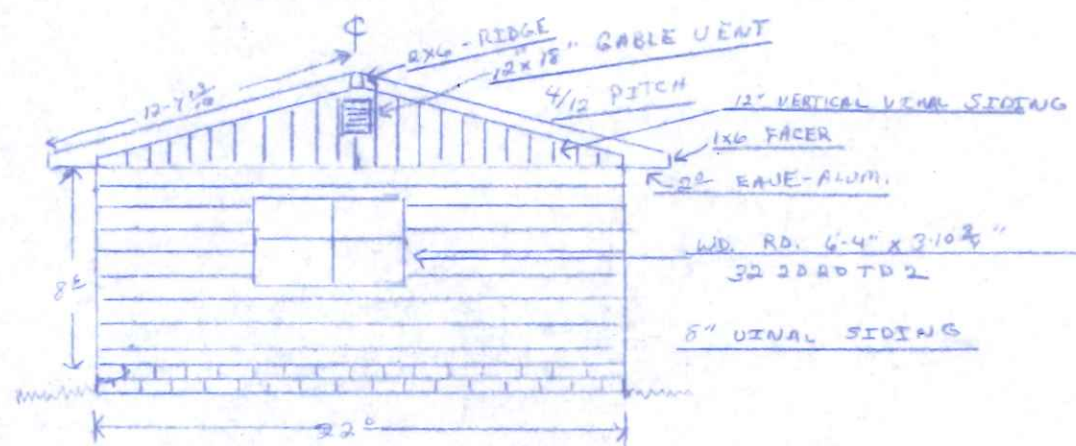
SOUTH ELEVATION
